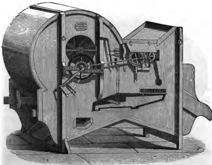
COOCH'S WINNOWING-MACHINE.
